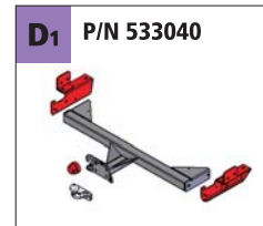
Rear towing device (for original bumper)
