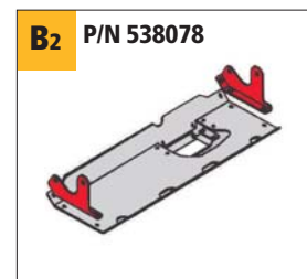
B2 P/N 538078 Front axle protector Cannot be mounted with B5
