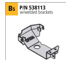
B5 P/N 538113 w/welded brackets Front and rear differential protector Cannot be mounted with B6, B8
