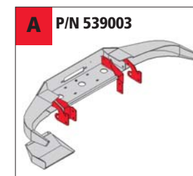
A P/N 539003 ATL HD winch bumper
