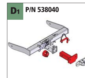
D1 P/N 538040 Detachable towing device
