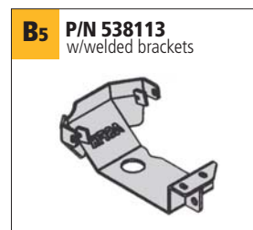
B5 P/N 538113 w/welded brackets Front and rear differential protector Cannot be mounted with B2, B6
