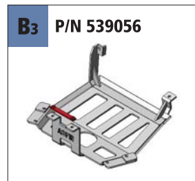
B3 P/N 539056 Rear Differential skid plate
