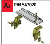
Winch mounting plate for original bumper
