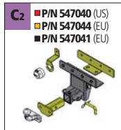
Gear/Transfer skid plate Fits veicle with lift kit up to 3"
