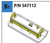
Steering rod protector for ATL HD bumper
